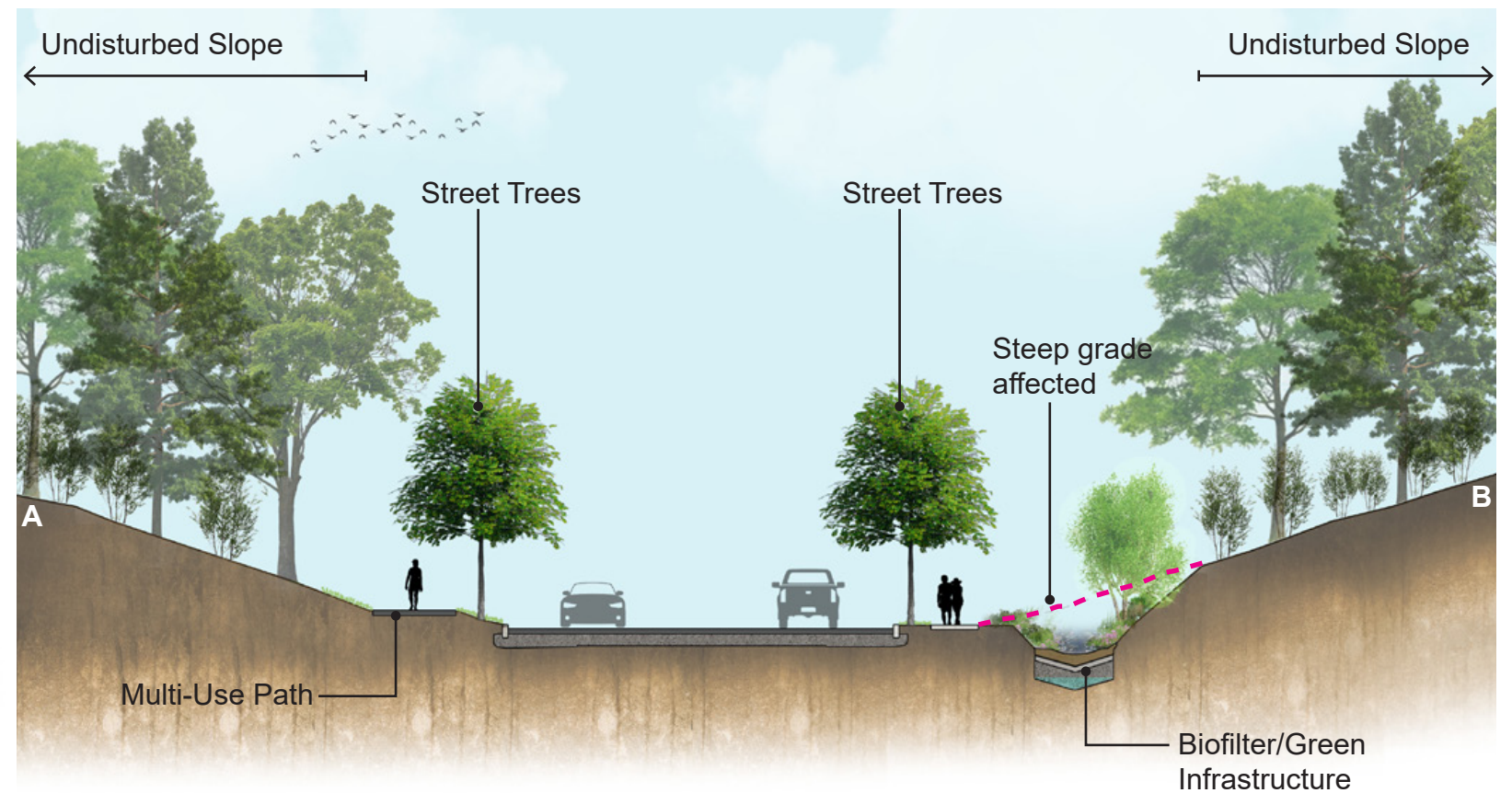
Entrance Road Section View
